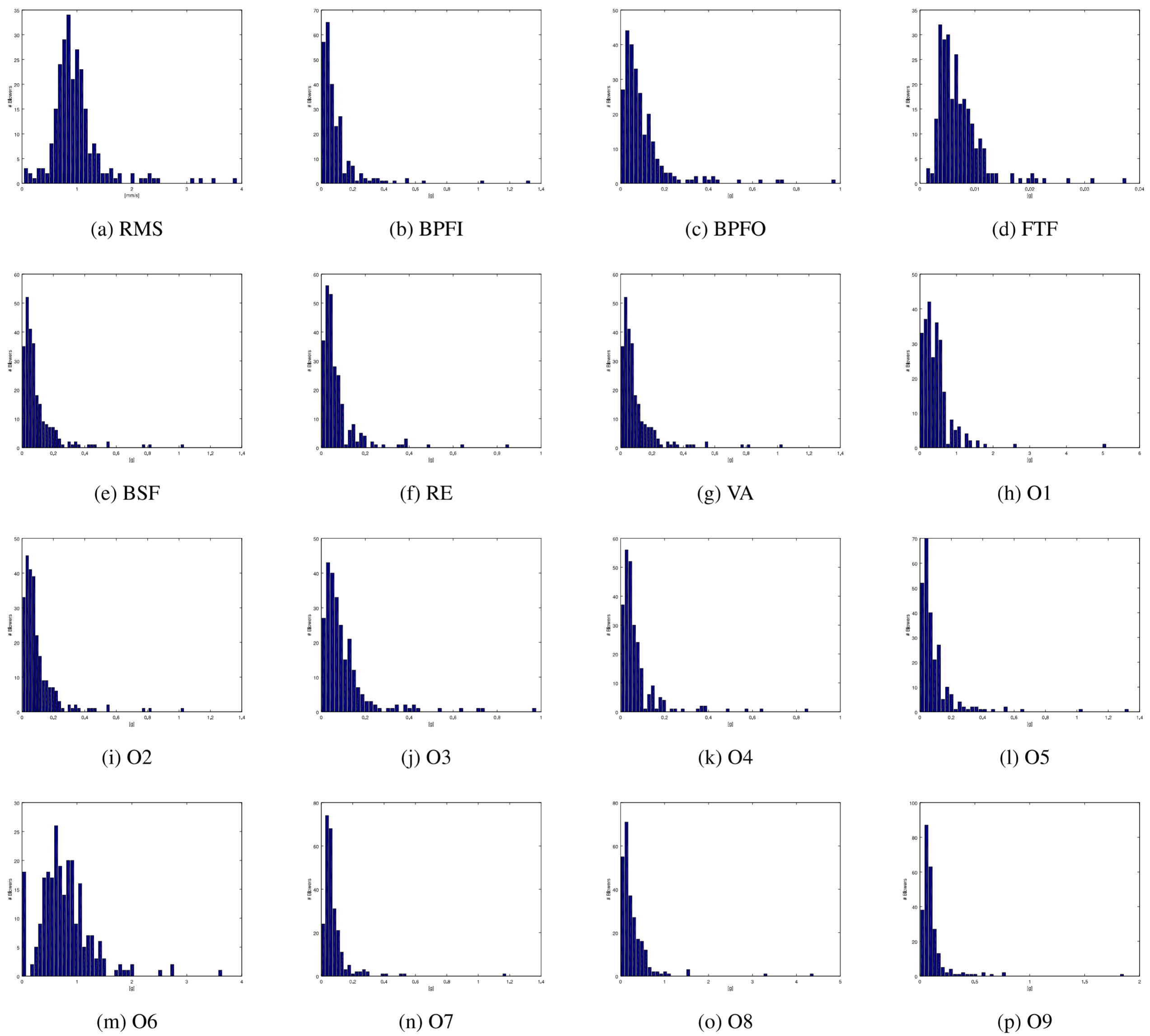
Figure 4. Statistical analysis of the indicators through the histogram.
