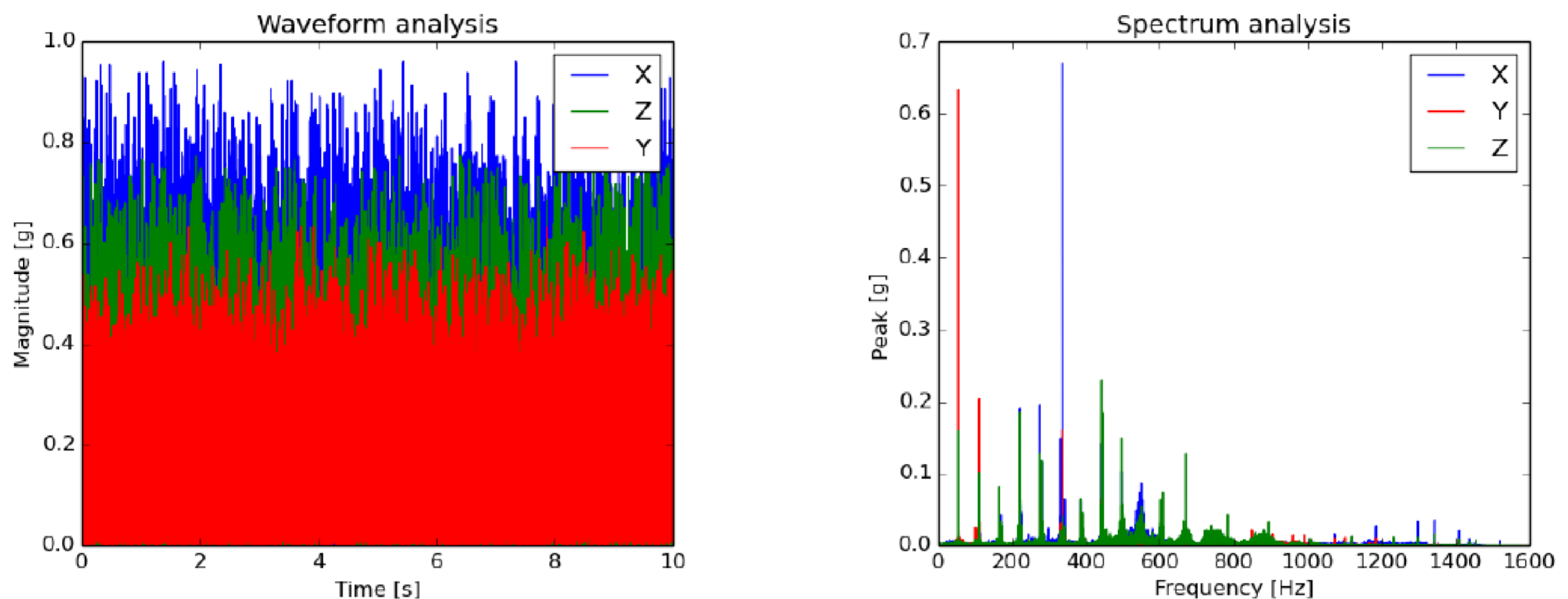
Figure 3. Example vibration signature of one traction-motor blower as it is acquired by TheMotes. Note the salient peaks on 55Hz and 330Hz. The axis with the greatest vibration amplitude (most severe fault) is selected for conducting the analysis.
