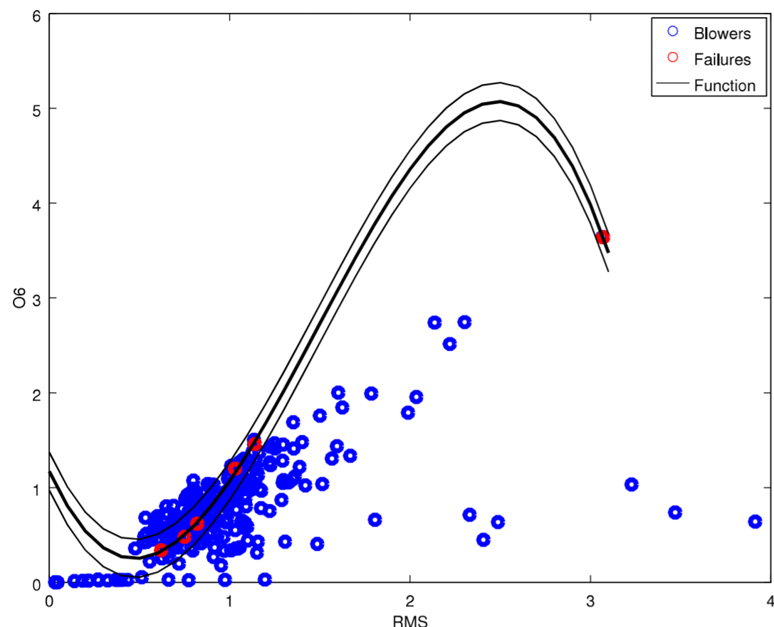
Figure 6. Indicator map and function learning.
