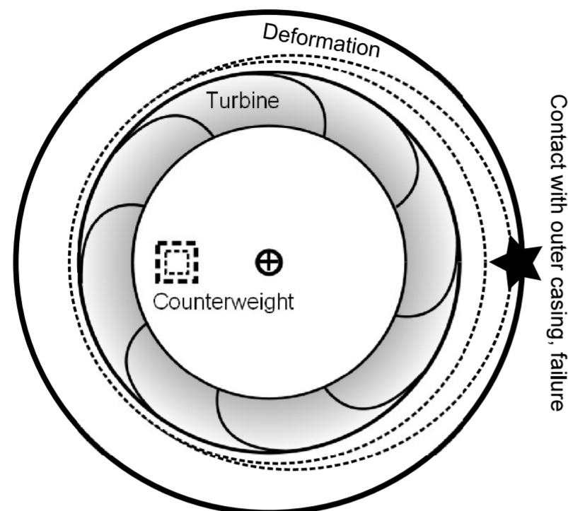
Figure 1. Fatigue of a traction-motor blower with counterweight imbalance corrections.
